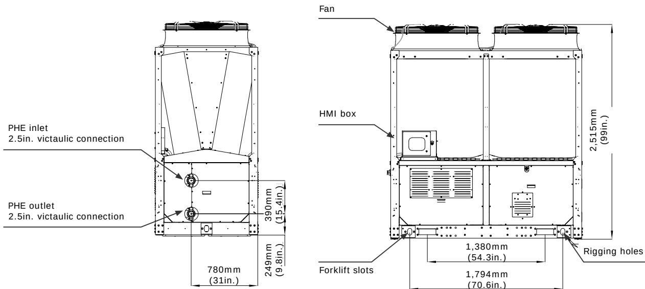
Piping connection side (QTH1 two-pipe unit)
