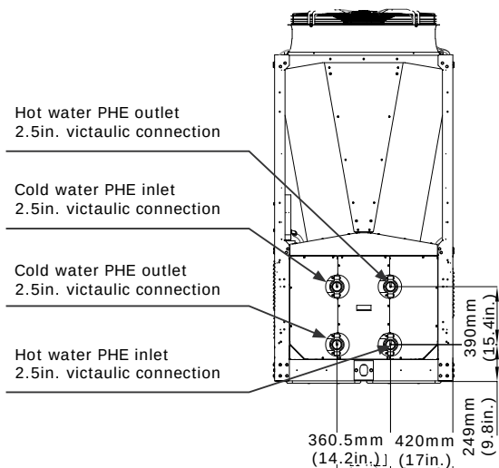
Piping connection side (QTH1 four-pipe unit)
